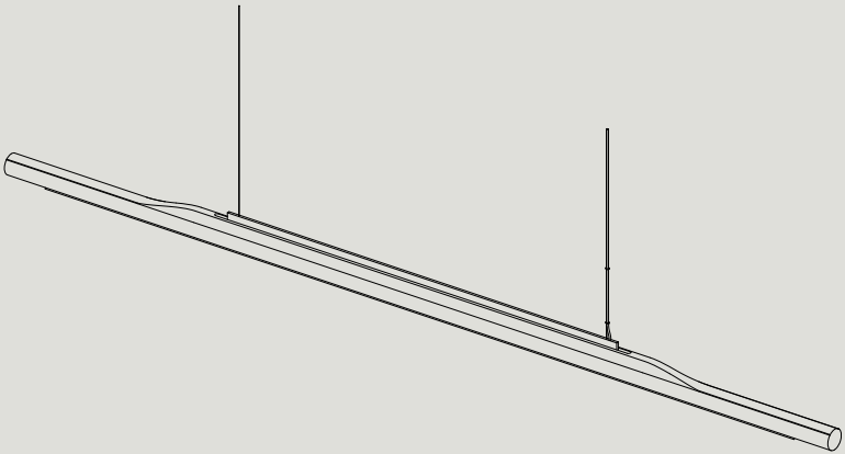
ALP.L L 2200 W 50 H 85 L 86" W 1.9" H 3.4" CEILING CANOPY SPACING L982 / 38.6"
