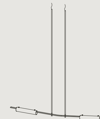
VC212 L 1790 W 70 H 100 L 70.5" W 3" H 4" MIN DROP HEIGHT - H 300 / 11.8"
