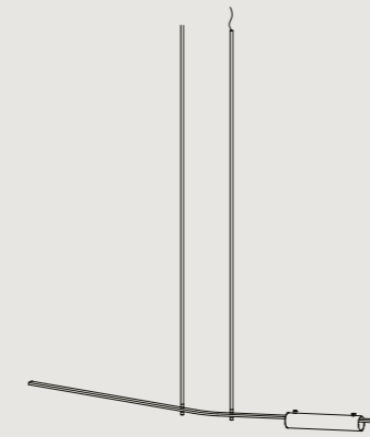
VC211 L 1790 W 70 H 100 L 70.5" W 3" H 4" MIN DROP HEIGHT - H 300 / 11.8"
